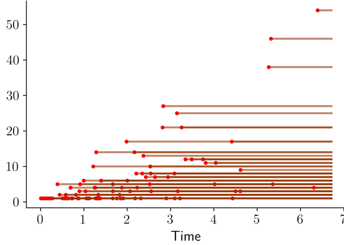
Figure 2: 100 realisations of \mathbf{W}_t generated using the Gillespie algorithm. \lambda = 1 , \mu = 0 , \delta = 0.1 .
