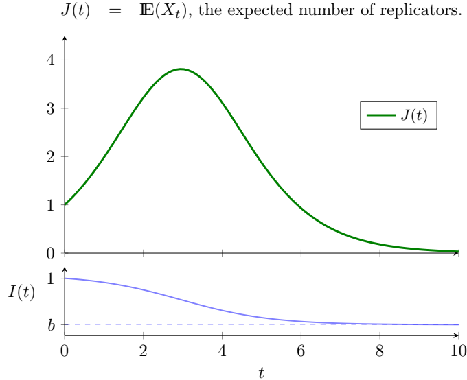
Figure 5: J(t) plotted against time. \lambda = 1 , \mu = 0.2 , \delta = 0.05 .
