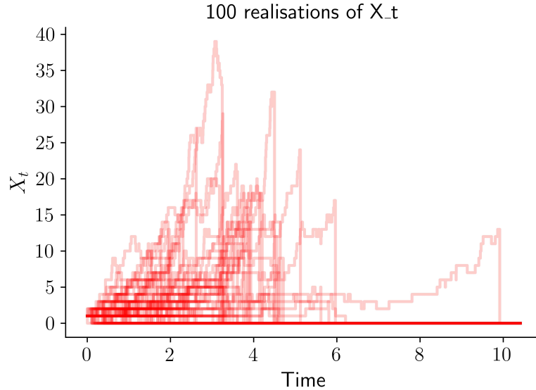
Figure 1: 100 realisations of \mathbf{X}_t generated using the Gillespie algorithm. \lambda = 1 , \mu = 0 , \delta = 0.1 .
