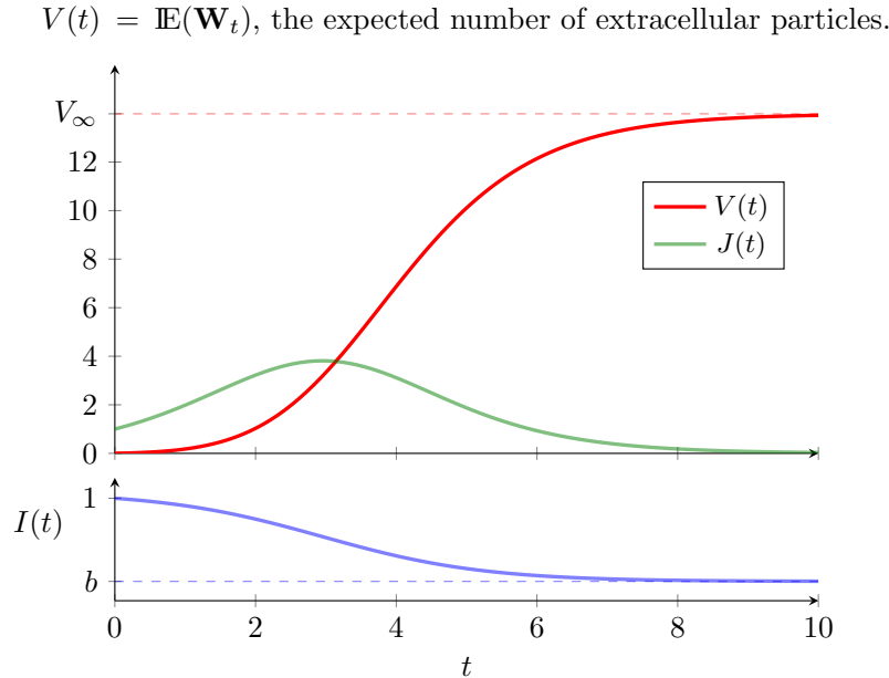
Figure 6: V(t) plotted against time. \lambda = 1 , \mu = 0.2 , \delta = 0.05 .
