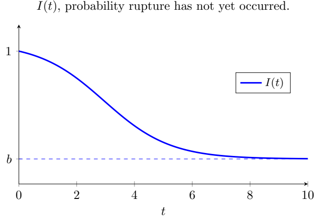
Figure 3: I(t) plotted against time. It converges to b , the probability that the process dies out internally before rupture. \lambda = 1 , \mu = 0.2 , \delta = 0.05 .
